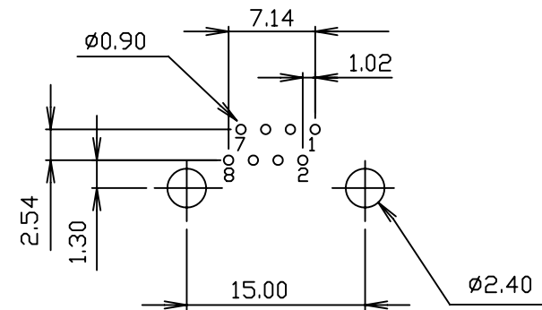
SUGGESTED PCB LAYOUT TOP VIEW
