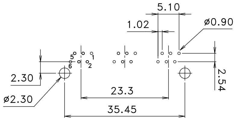
SUGGESTED PCB LAYOUT TOP VIEW
